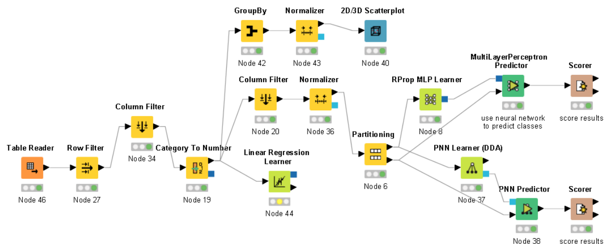
Figure 5: Neural Network Model
