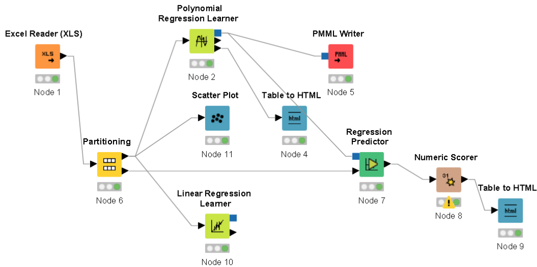
Figure 3: Initial Polynomial and Linear Regression
